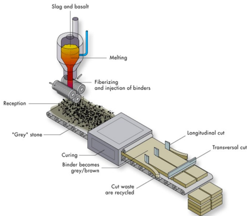
Figure 3. Traditional process of stone wool production (Eurima 2, 2011)
